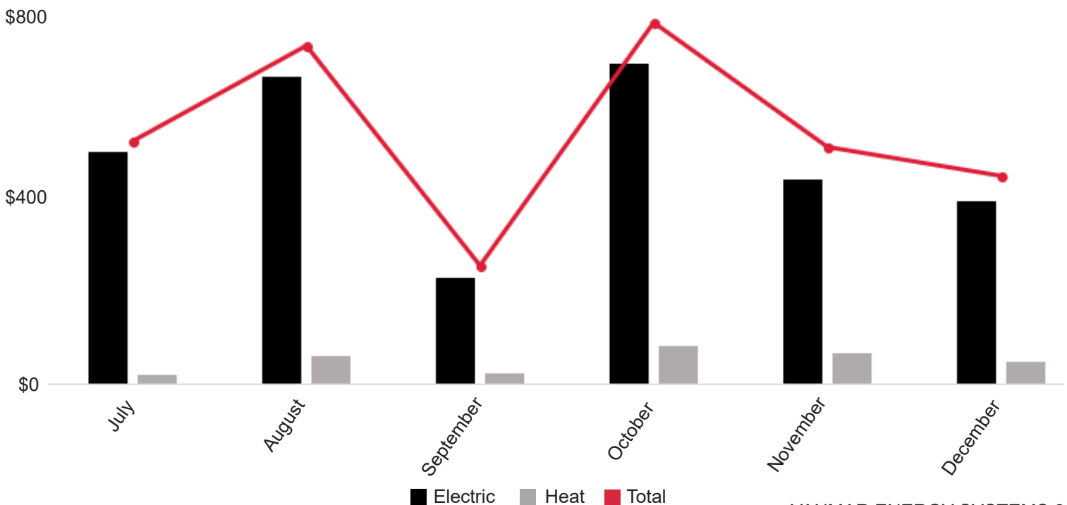
YANMAR CHP Savings - July through December 2017
