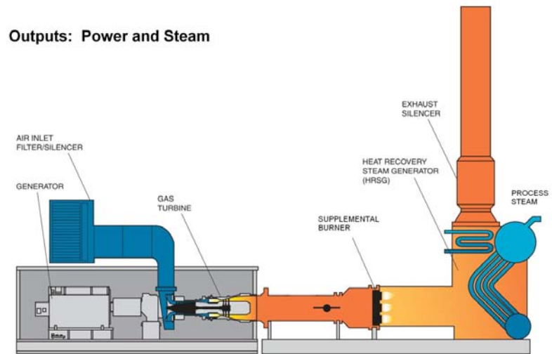
Figure 1. Diagram of the Frito-Lay combined heat and power (CHP) system
